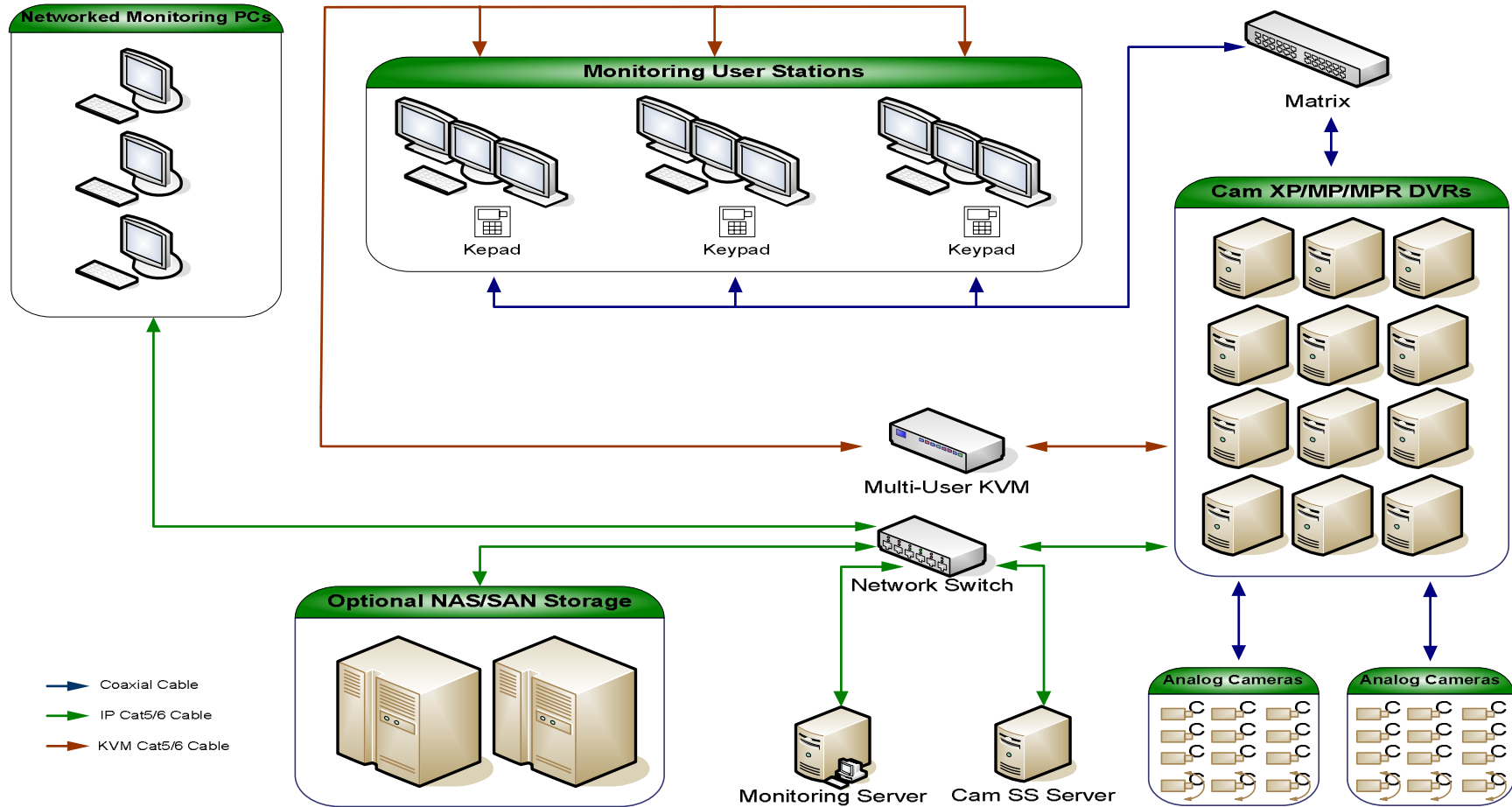
Digital Video Recording System Network Diagram (DVRs before Matrix Switcher Configuration)
